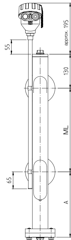
NBK-... with Transmitter - Option H (not possible with option VA)
