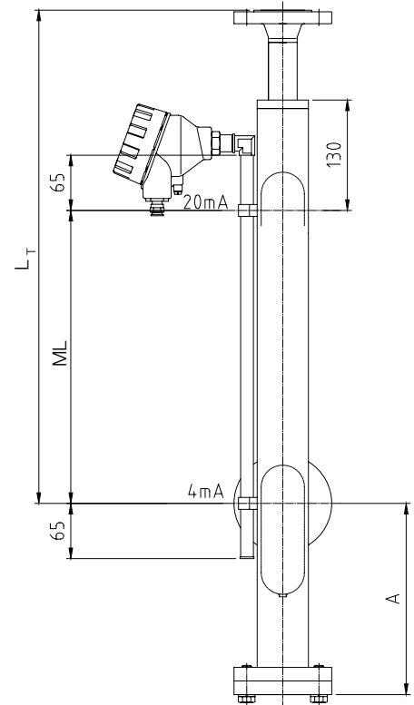
NBK-... with Transmitter - Model H - Option ST
