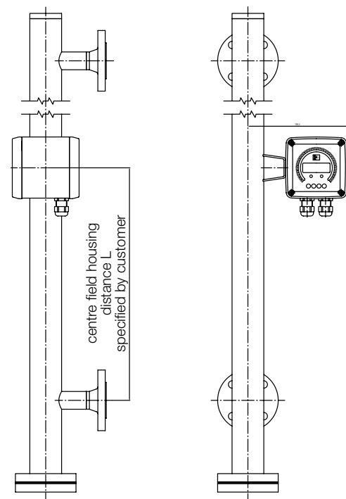
NBK-... with Indication Unit ADI-1 - Option C
