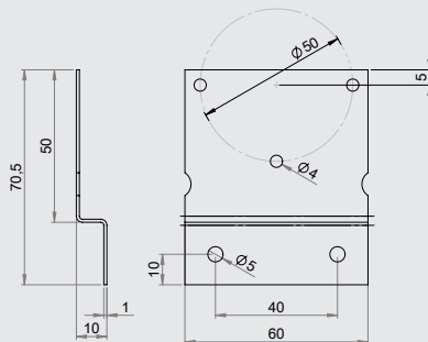
Mounting bracket 4202
