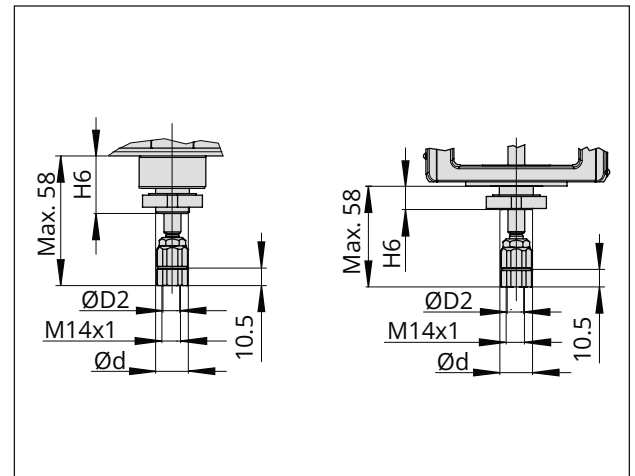
Fig. 28: Type 3271-5 and Type 3277-5 with 7.5 mm travel for Type 3510 Micro-flow Valve
