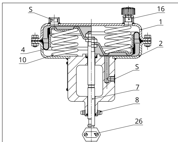
Fig. 9: Type 3277 for direct attachment of accessories (example shows actuator with 350 cm 2 )
