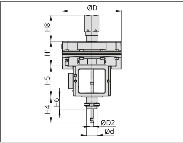
Fig. 22: Type 3277-5 with travel stop
