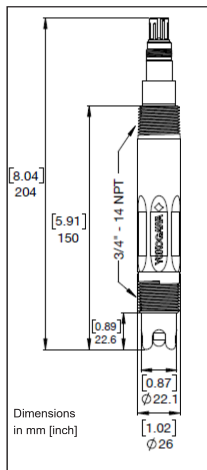
Figure 4: Dimensions PH21
