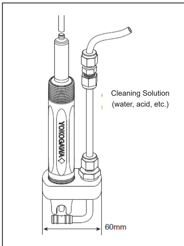
Figure 5: Installation example using spare part K1547PJ
