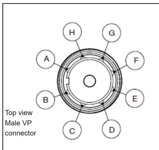
Figure 3 : Connection diagram
